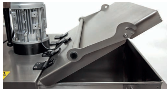
Tank cover with EasyStop hinges
